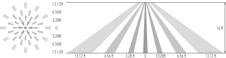
Mounting height < 16 ft (5 m) ceiling mounted.
