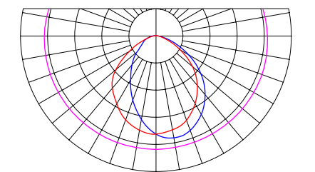
luminous intensity distribution diagram
