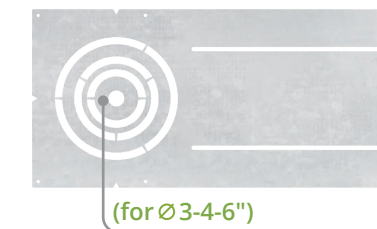
ASD-MPL-FA WITH ASYMMETRIC HOLES
