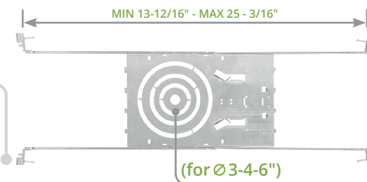
ASD-MPL-SC WITH SLIDING CLIPS
