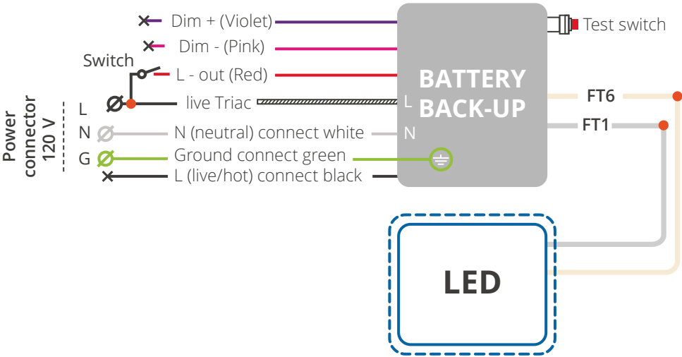
WIRING DIAGRAM (120VAC TRIAC DIMMABLE)
